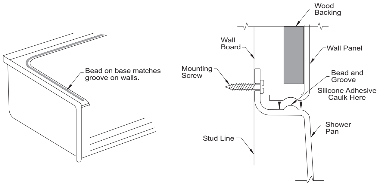
BASE / WALL MATING DETAIL
